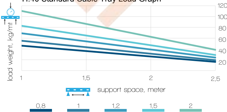
H:40 Standard Cable Tray Load Graph
