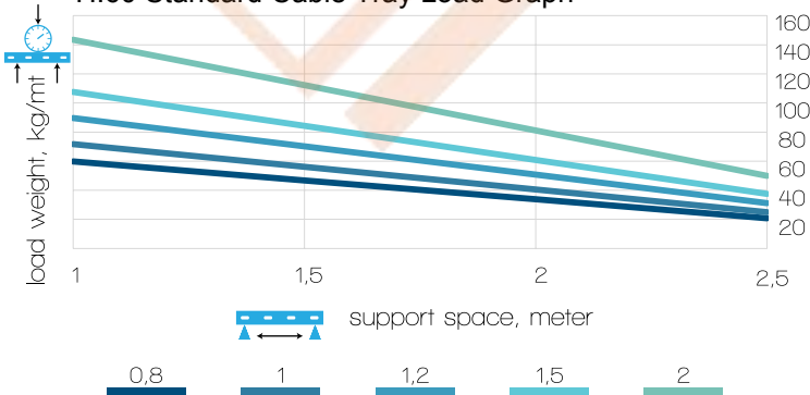
H:60 Standard Cable Tray Load Graph
