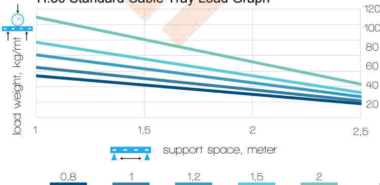
H:50 Standard Cable Tray Load Graph
