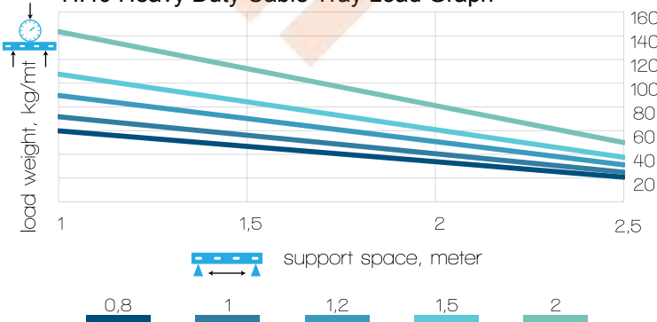
H:40 Heavy Duty Cable Tray Load Graph
