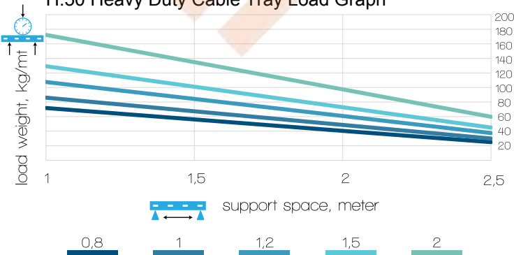
H:50 Heavy Duty Cable Tray Load Graph
