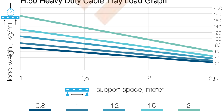
H:50 Heavy Duty Cable Tray Load Graph
