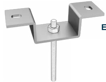
Tavan Tespit (Omega Tipi) Threaded Rod Head Plate (Omega Type)
