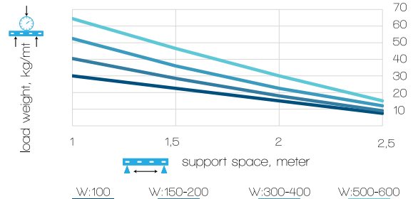
H:35 Wire Mesh Cable Tray (T:5.0mm) Load Graph
