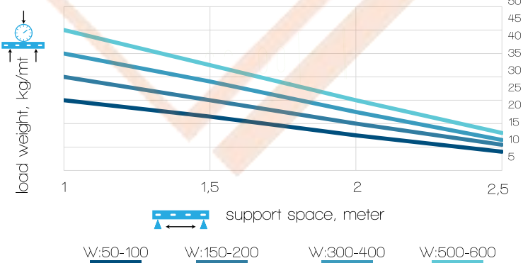
H:60 Wire Mesh Cable Tray (T:4.0mm) Load Graph
