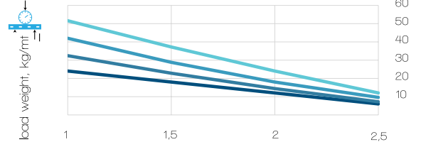
H:35 Wire Mesh Cable Tray (T:5.0mm) Load Graph
