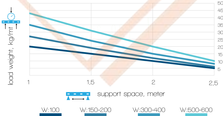
H:35 Wire Mesh Cable Tray (T:4.0mm) Load Graph
